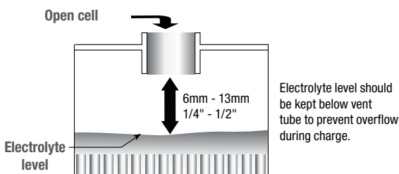
FIGURE 7: Electrolyte level
