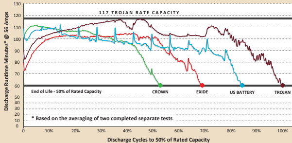
INDEPENDENT LABORATORY TESTING - 8V BATTERIES
